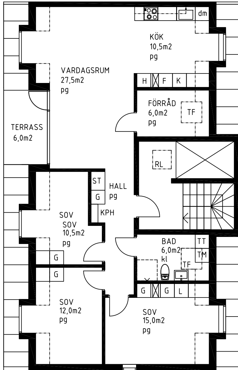
PLAN 4
